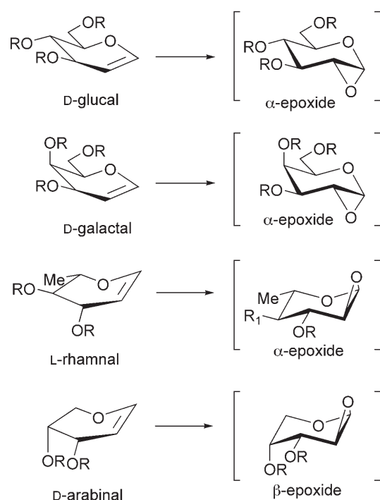
Figure 4. Favoured intermediate epoxides.
