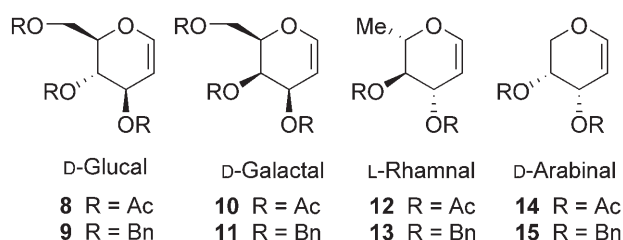
Figure 3. Glycols used as substrates for the catalyzed domino epoxidation-methanolysis.
