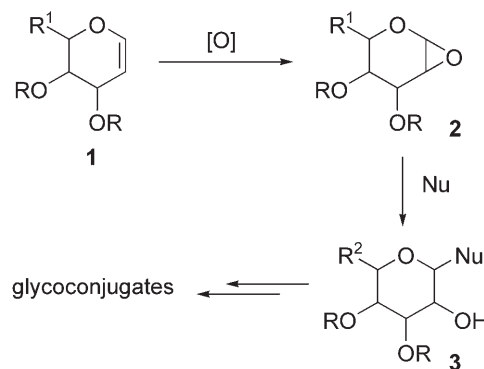
Scheme 1. Synthetic sequence for use of glycals as building blocks in the construction of glycoconjugates.
