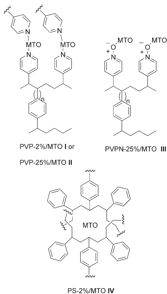
Figure 1. Structures of poly(4-vinylpyridine)/MTO and polystyrene/MTO catalysts I–IV .
