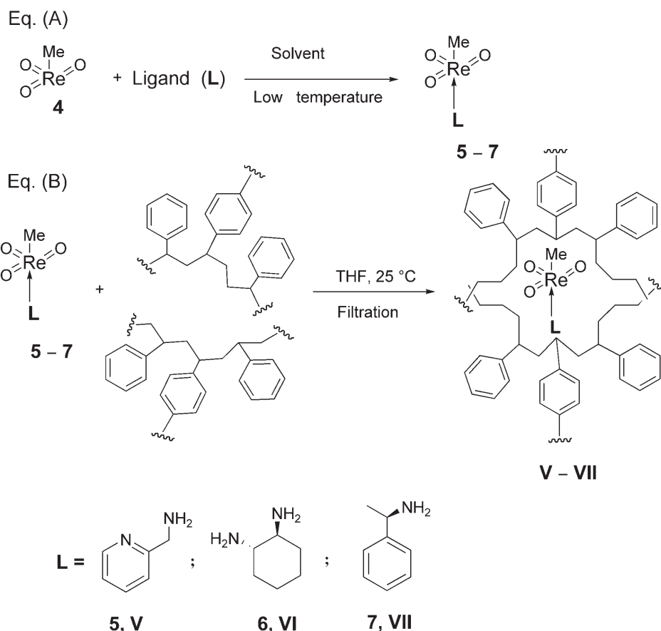
Figure 2. Lewis bases-MTO adducts 5–7 and microencapsulated PS 2%/MTO-Lewis base adducts V–VII used as catalysts.
